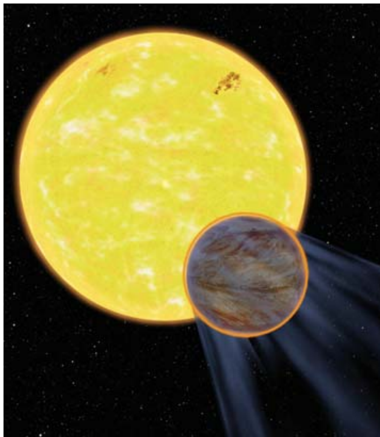
SILHOUETTE OF A PLANET, shown in this artist's conception, is inferred from Hubble measurements of the brightness of the host star.
