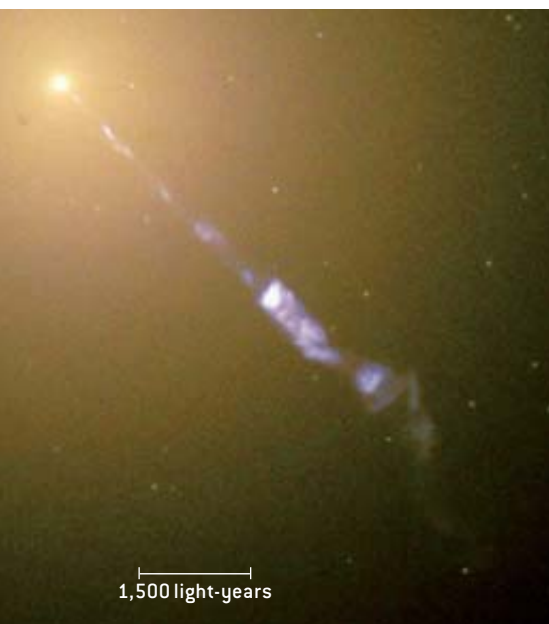
PLASMA JET, thought to be generated by an accreting black hole of three billion solar masses, squirts out of galaxy M87.
