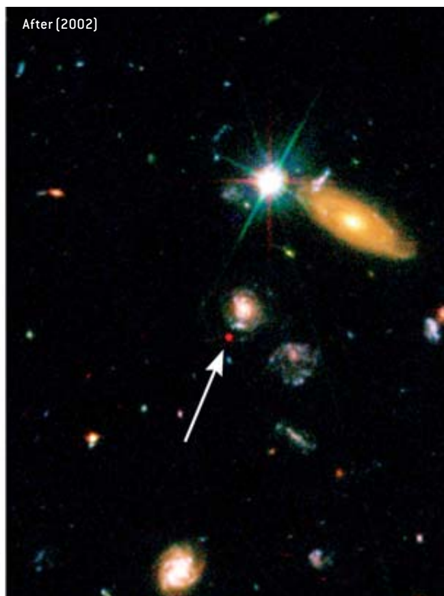
DISTANT SUPERNOVA, discovered by comparing images from different times, helped to reveal a momentous transition from cosmic deceleration to acceleration.
